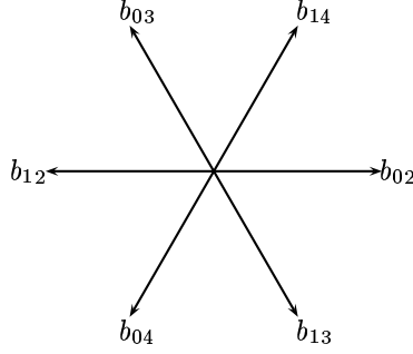
Figure 4: Transpose of the matrix B
