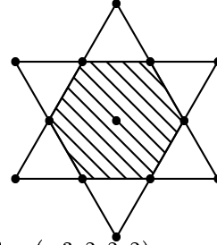
Figure 6: Monomials in multidegree \theta = (-3, 2, 2, 2)
